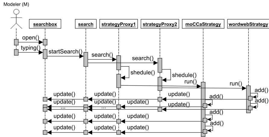
Fig. 5. Sequence Diagram: search()
